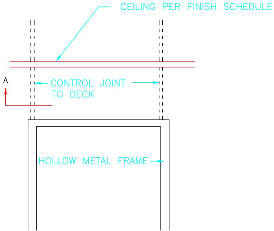
PARTITION - CONTROL JOINTS AT DOOR
