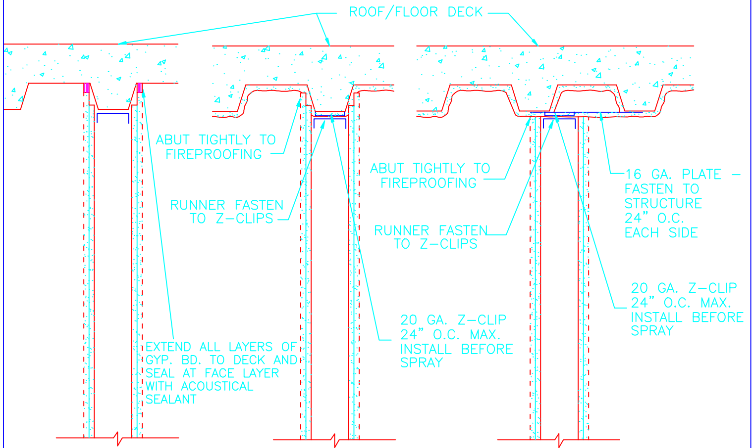
RATED PARTITION - PARALLEL TO CONCRETE DECK FLUTES WITH SPRAY-ON FIREPROOFING
