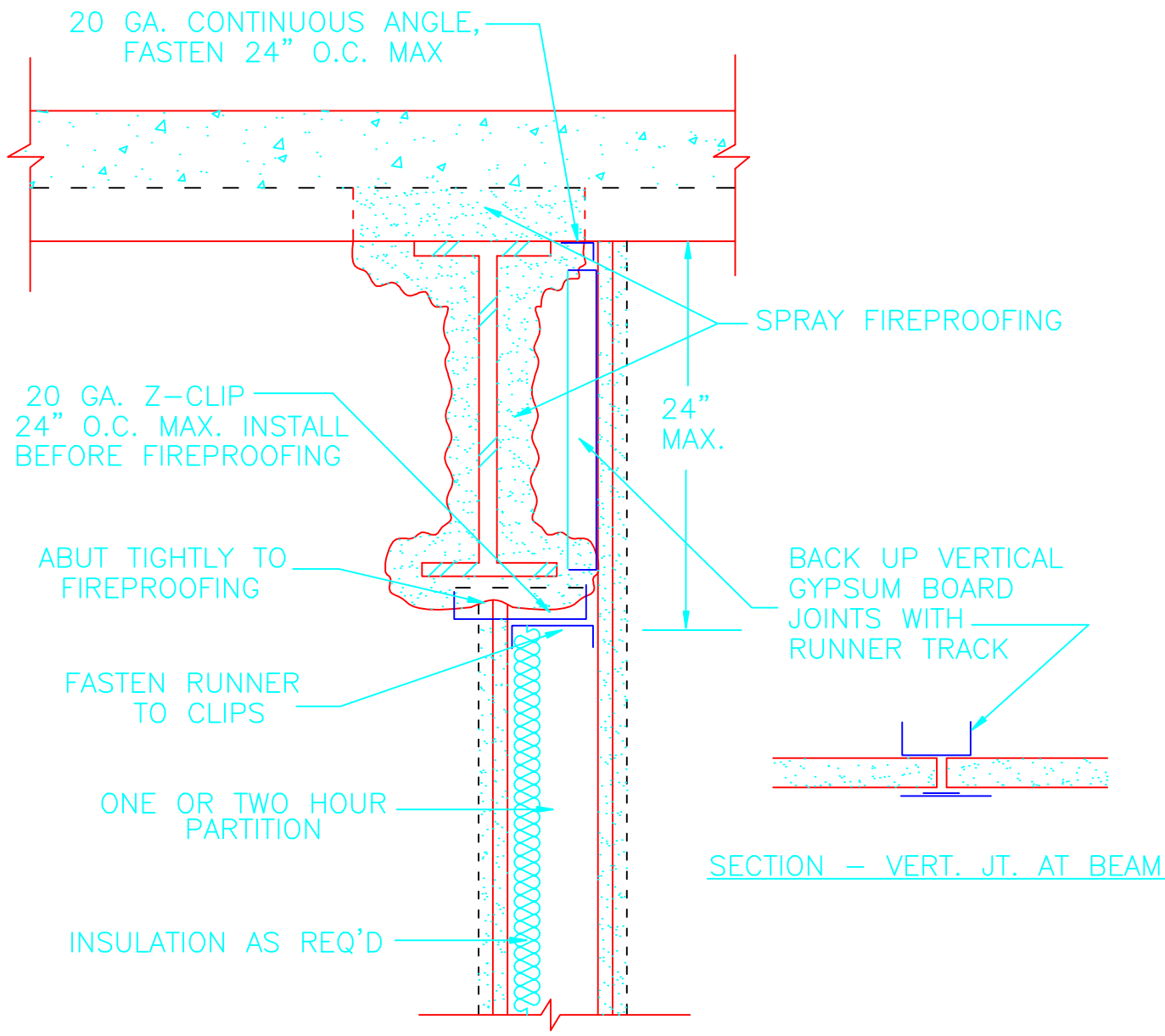
RATED PARTITION - UNDER BEAM
