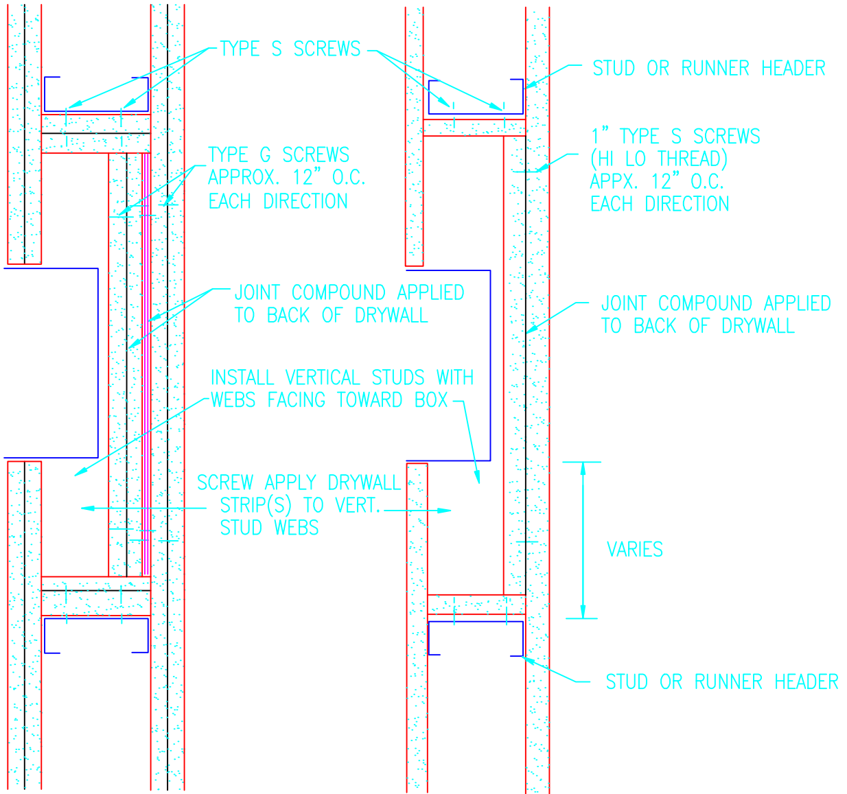
SECTION - TWO HOUR WALL
