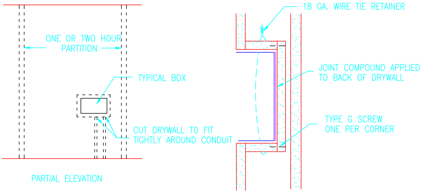
SECTION - ONE HOUR WALL
