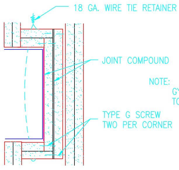
SECTION - TWO HOUR WALL
